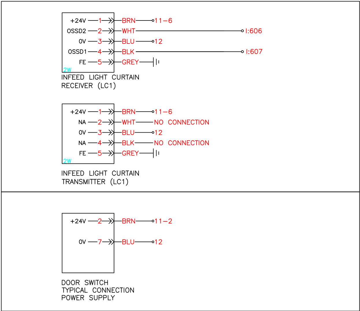
INFEED LIGHT CURTAIN
